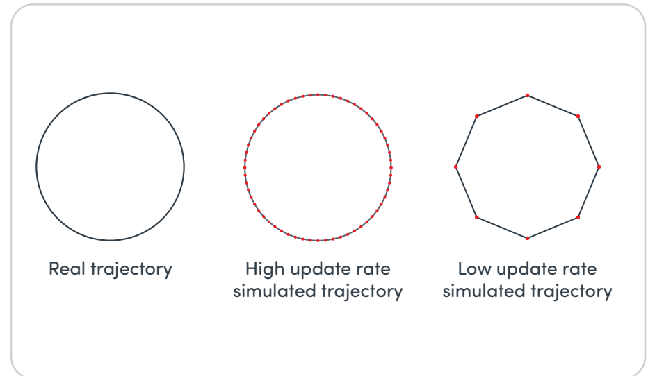
Vehicle circular motion at different update rates
